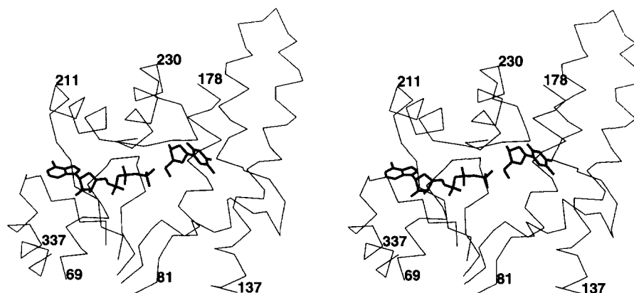
Fig. 3. Stereo-view of the C_{\alpha} -backbone around the active center together with the bound substrates thymidine and ATP. Presented are five polypeptide segments, all starting at the carboxy-terminal end of the parallel 5-stranded \beta -sheet. The segments starting at positions 52, 80, 160, 202, and 324 contain \alpha -helices a1, a2 & a3 and part of a4, a5, a7 and part of a8, and a10, respectively. The glycine-rich loop encircles the \beta -phosphoryl group of ATP.
