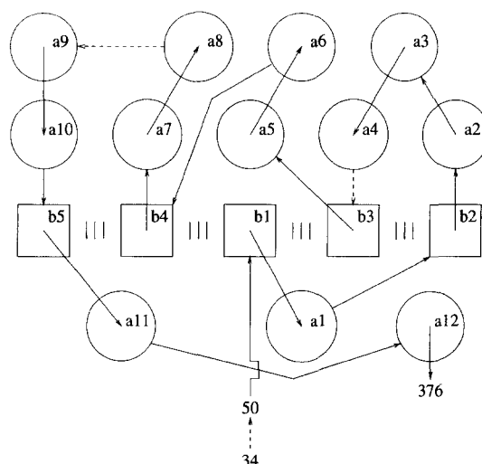
Fig. 1. Sketch of the chain fold of thymidine kinase from Herpes simplex virus type 1. To avoid crossovers the sketch is somewhat simplified rendering some helix positions disputable. All \beta -strands (quadrangles) run towards the viewer, the orientations of the helices (circles) are indicated by the arrows. Dashed lines denote chain segments that are not yet modeled. The central residues of secondary structure elements b1, b2, b3, b4, b5, a1, a2, a3, a4, a5, a6, a7, a8, a9, a10, a11, and a12 are 52, 79, 159, 203, 326, 67, 87, 103, 131, 172, 190, 215, 239, 292, 314, 340, and 364, respectively.
